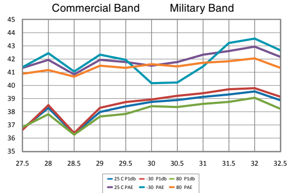
Figure 2. Output P1dB & PAE
